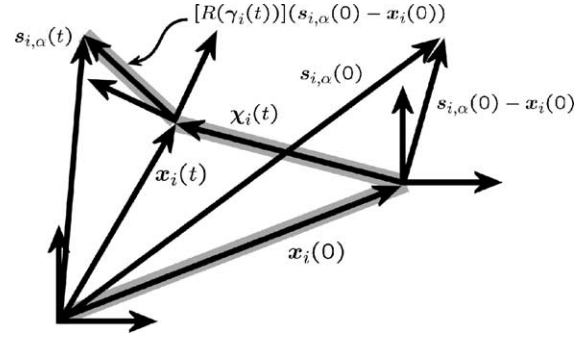
Fig. 2. This 2D representation shows the relationship between all quantities used to describe the position of \mathbf{s}_{i,\alpha}(t) . Eq. (14) can be derived from this figure by summing all vector quantities along the shaded path.
