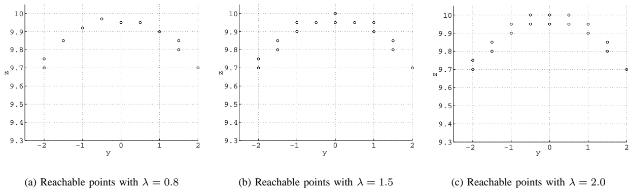
Fig. 5. Reachable points in the y-z Plane
