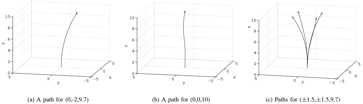
Fig. 4. Paths by inverse kinematics with \kappa = 0.05 and \lambda = 0.8
